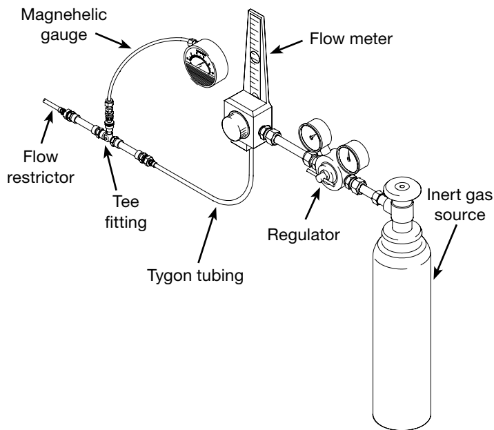
Internal Purge Pressure Kit for 1/4, 3/8, and 1/2 In. Tubing
